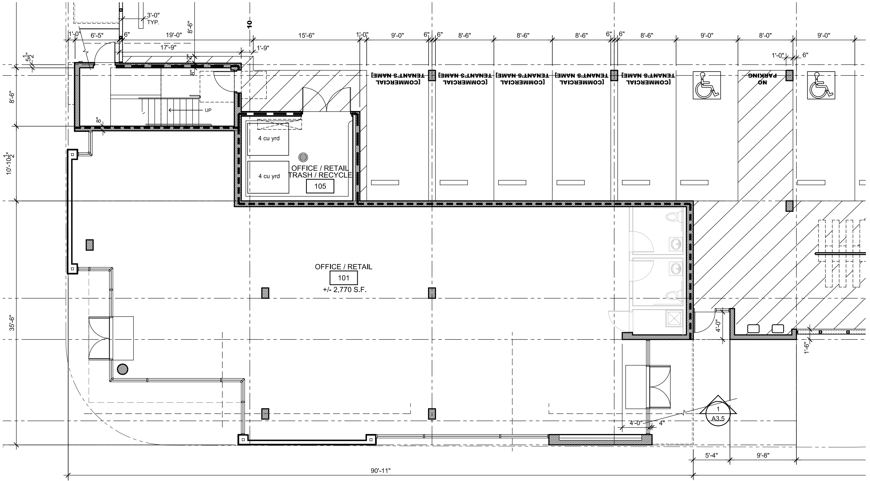
1 OFFICE / RETAIL SPACE SCALE: 1/8" = 1'
